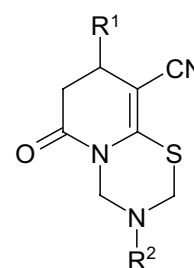
Figure 1. Formulas of test substances. I: R^1 = 3,4,5-(\text{MeO})_3\text{C}_6\text{H}_2 , R^2 = \text{Bn} ; II: 2-MeOC 6 H 4 , 2-EtC 6 H 4 ; III: 2-MeOC 6 H 4 , 3-Cl-4-MeC 6 H 3 ; IV: 3,4,5-(MeO) 3 C 6 H 2 , 2-FurCH 2 ; V: 3-MeO-4-EtOC 6 H 3 , 4-ClC 6 H 4 .
