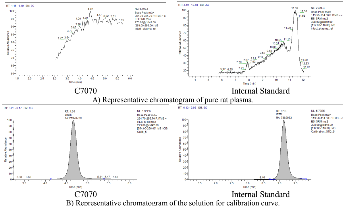
Figure 1. Representative chromatograms in determining the selectivity.
